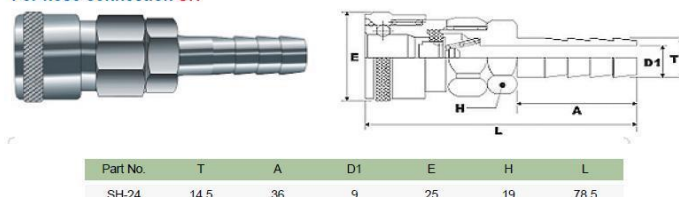
For hose connection SH
