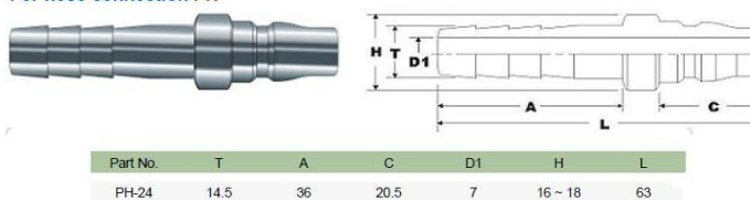
For hose connection PH
